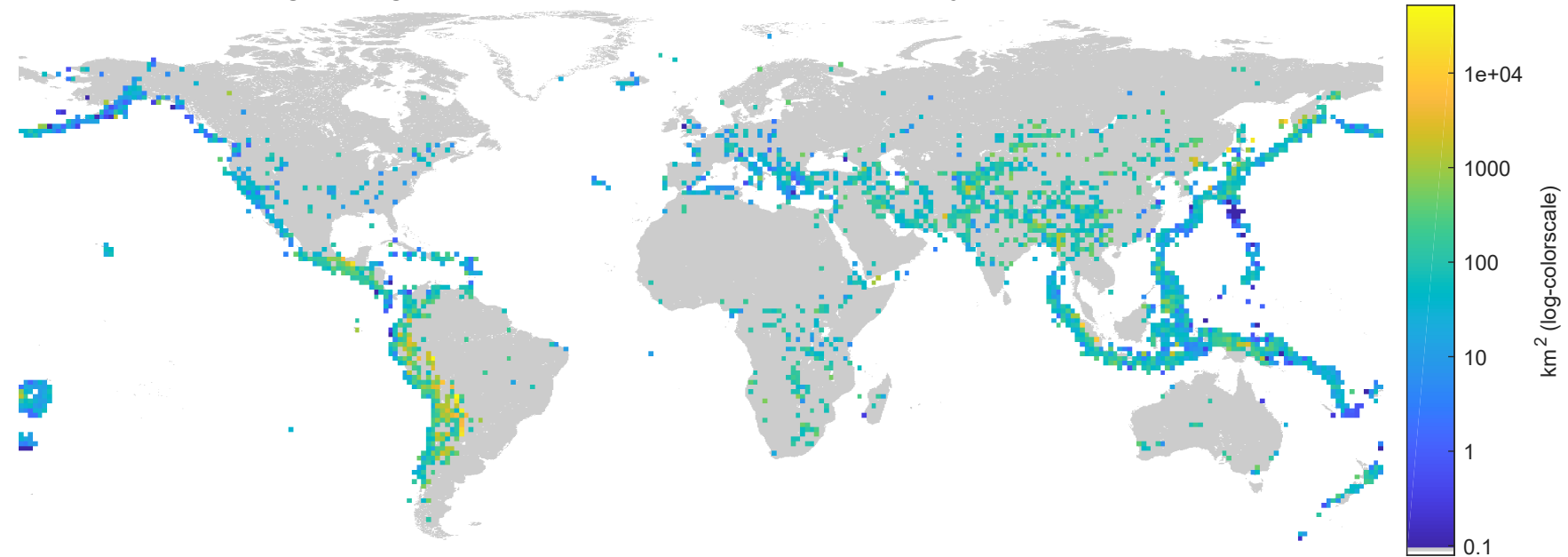
Average strong motion area (with 90 % of maximum PGA) by epicenter location
