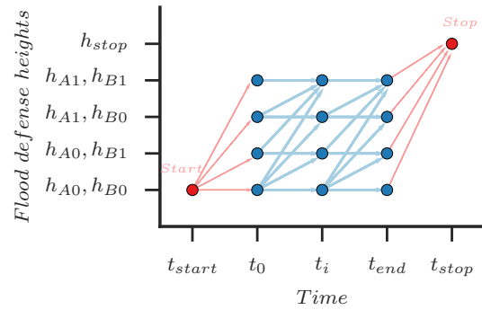
Figure 6. The graph of Fig. 5 with an additional stop vertex.
