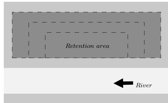
Figure 22. A retention area can also be optimised using the approach proposed in this paper. In this example, the surface area of the retention basin is used instead of the height of a flood defence.
