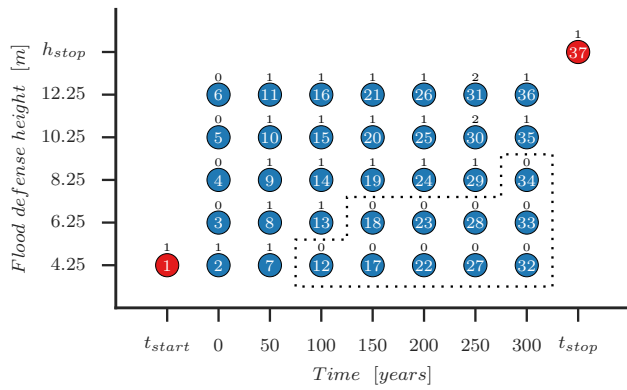
Figure 14. Number of times each vertex is visited by the algorithm for the example in Sect. 2.2. The dotted area emphasises that a part of the graph is never visited, while vertices 30 and 31 get visited twice.
