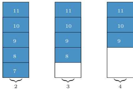
Figure 12. The adjacency lists for vertices 3 and 4 of Fig. 7 are reduced sets of the adjacency list for vertex 2.
