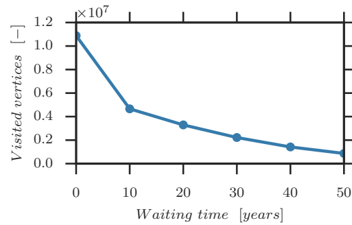
Figure 13. Total number of visited vertices as a function of the waiting time for the example of Sect. 4.3.
