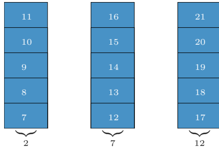
Figure 11. The adjacency lists for vertices 7 and 12 of Fig. 7 can be obtained by adding an offset to the adjacency list of vertex 2.
