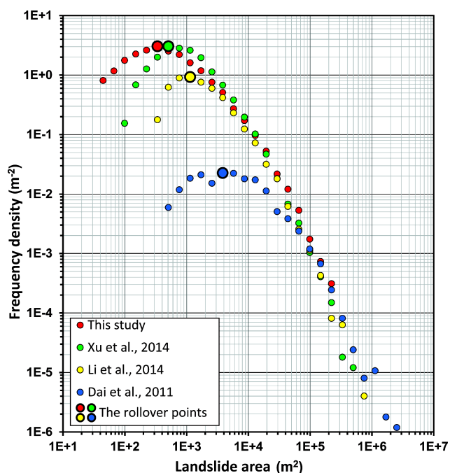
Figure 6. The frequency–area distributions (FAD) of the different co-seismic landslide inventories collected for the study area.
