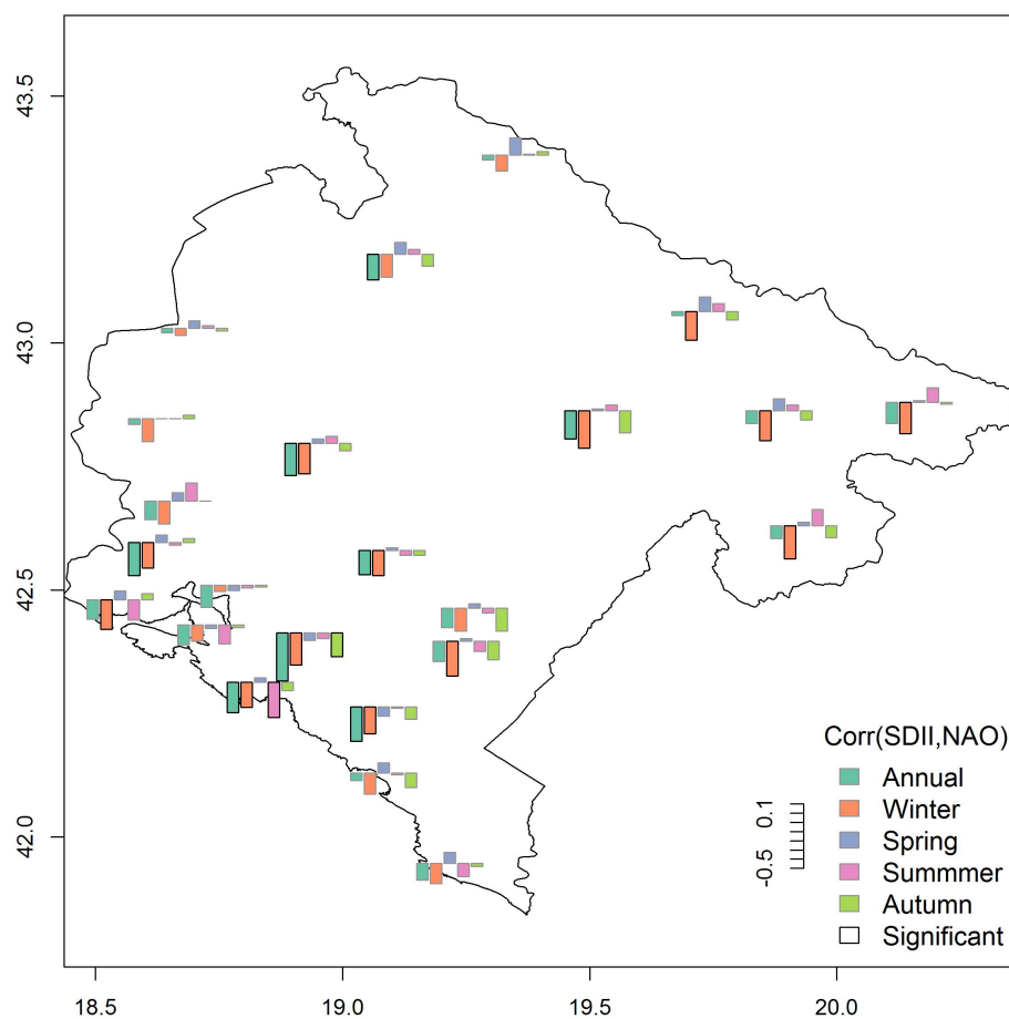
Fig. S1. Mapped correlation between annual and seasonal SDII and NAO index
