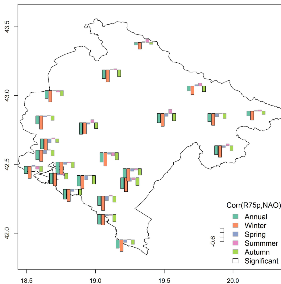
Fig. S3. Mapped correlation between annual and seasonal R75p and NAO index
