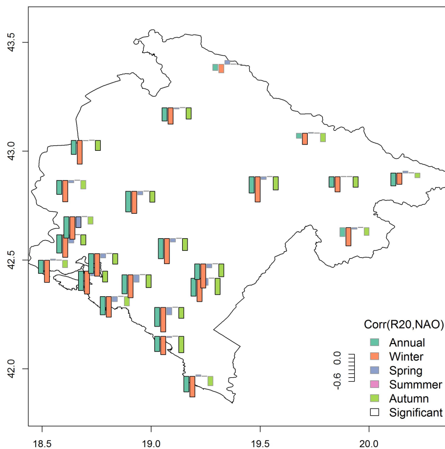
Fig. S4. Mapped correlation between annual and seasonal R20mm and NAO index
