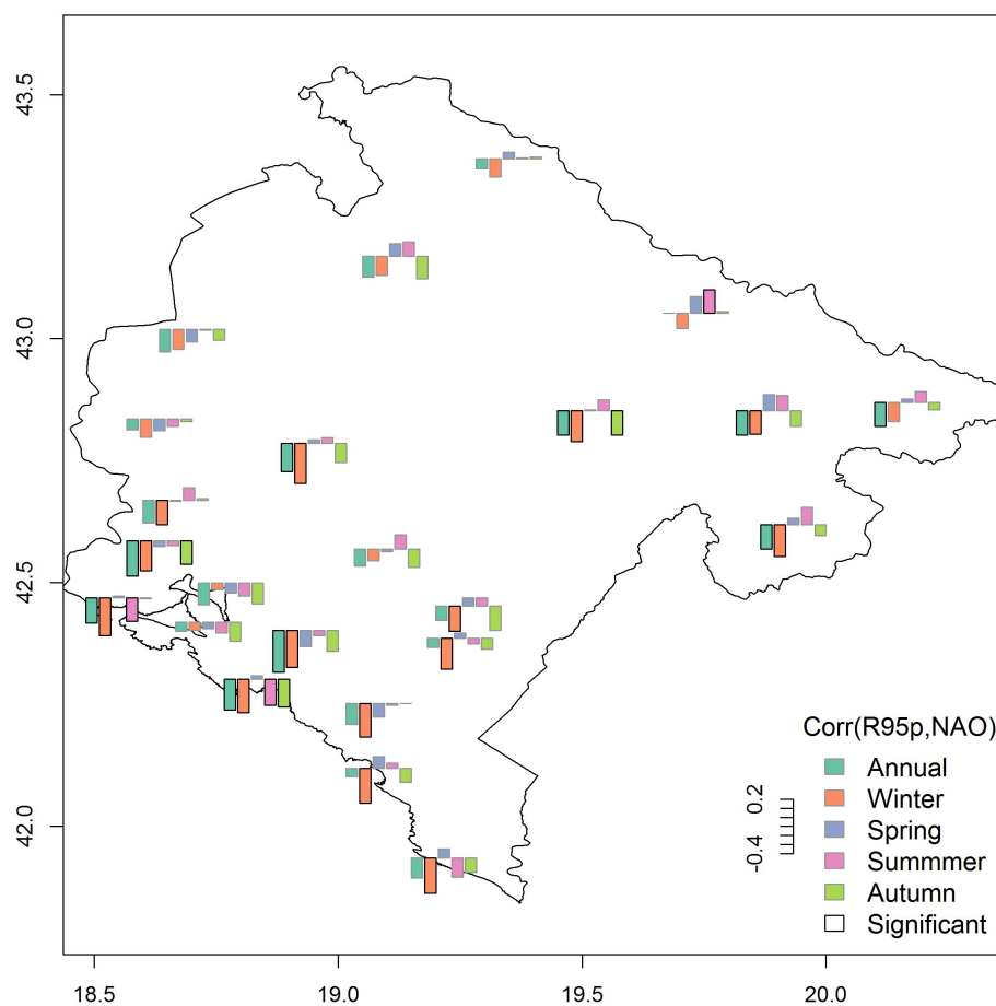
Fig. S2. Mapped correlation between annual and seasonal R95p and NAO index
