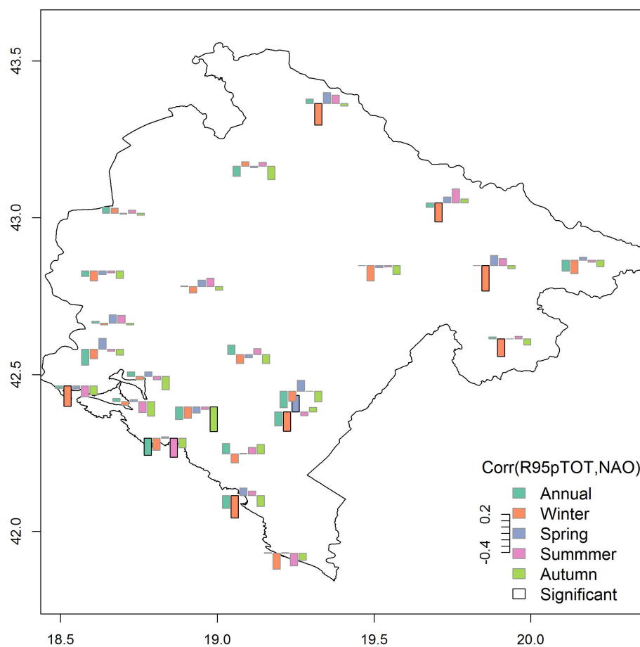
Fig. S5. Mapped correlation between annual and seasonal R95pTOT and NAO index
