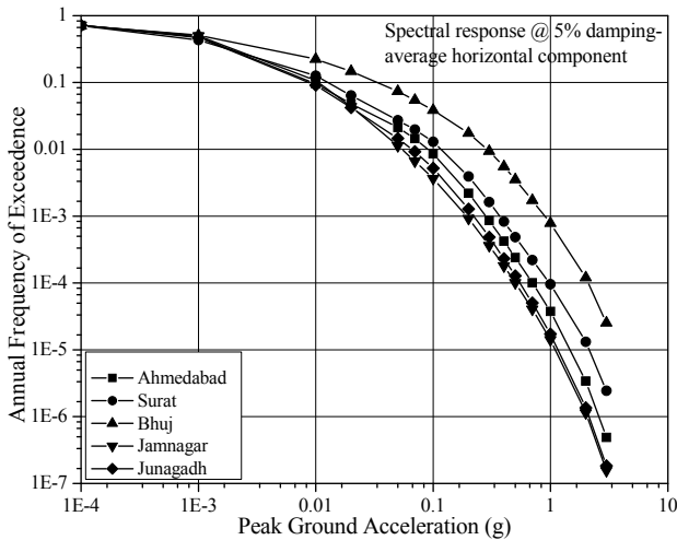
Fig. 11. Total Hazard calculated for various cities at zero spectral period i.e. PGA.
