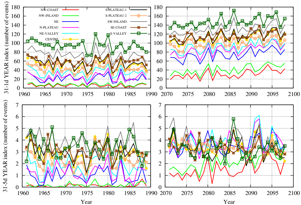
Fig. 4. Time series of extreme T_{max} climatic indices (YEAR, annual impact from October to September) for irrigated spring wheat at locations of Fig. 1. Left column shows results for the current climate and right column for the future scenario A2. Upper plots show the number of events with 1 day over the threshold of 31 °C (31-1d), and below, the number of events with 5 consecutive days over 31 °C (31-5d) are shown. Values correspond to the ensemble mean.
