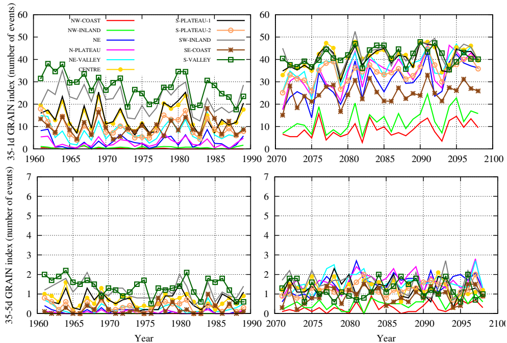
Fig. 5. Time series of extreme T_{max} stress indices of effective impact during grain filling (GRAIN) for maize at locations of Fig. 1. Left column shows results for the current climate and right column for the future scenario A2. Upper plots show the number of events with 1 day over the threshold of 35 °C (35-1d), and below, the number of events with 5 consecutive days over 35 °C (35-5d) are shown. Values correspond to the ensemble mean.
